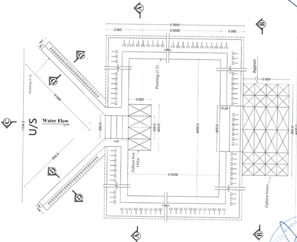
Plan of Water storage SCALE : N .TS
